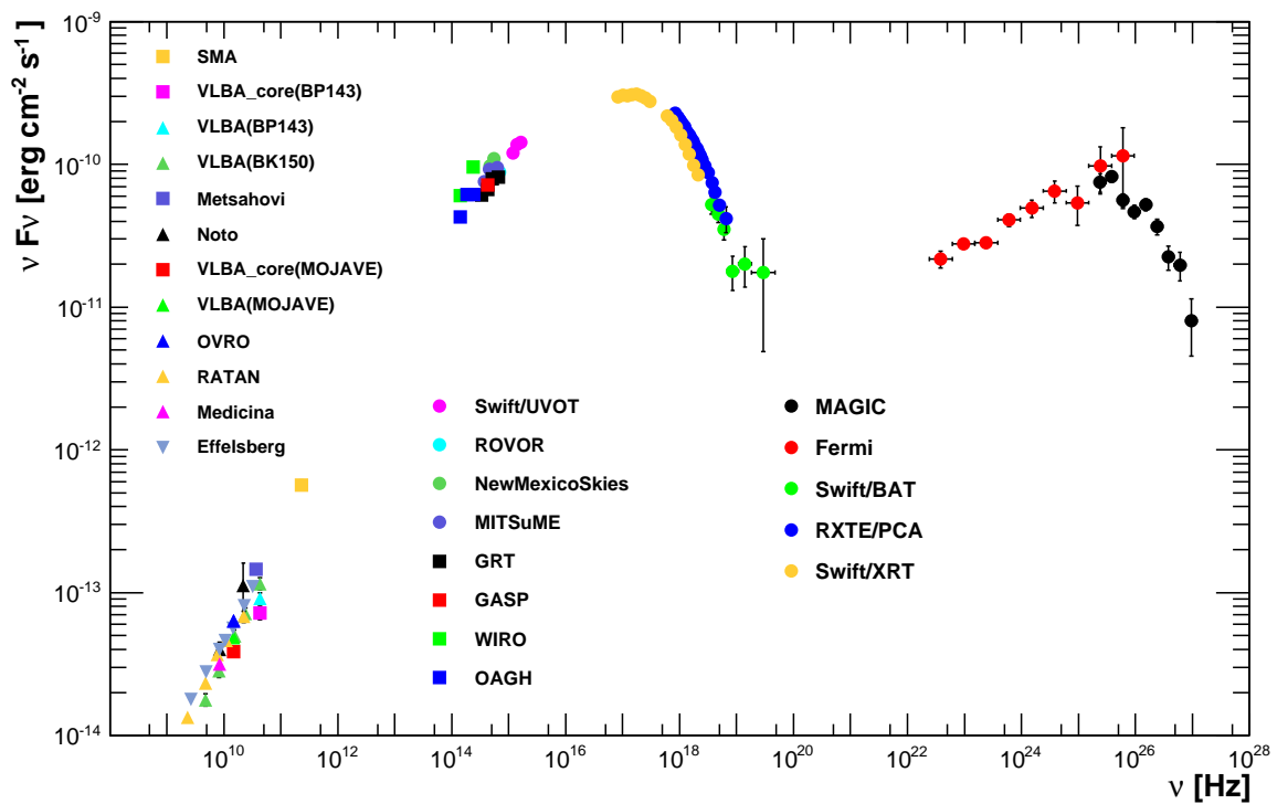
Figure 3.1 Spectral energy measurements for the blazar Markarian 421, showing the low hump in 10^9 to 10^{20} Hz, and the high-energy hump from 10^{20} to 10^{28} Hz, including data taken from radio, infrared, optical, ultraviolet, x-ray and gamma-ray observatories. Figure from [49].
