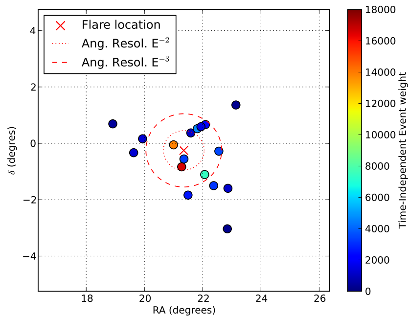
Figure 9.10 The 17 most significant events seen from the 59-string most significant flare location with their sky coordinates and time-independent event weights. The flare location is marked with an X, along with the median angular resolution for two different signal spectra.
