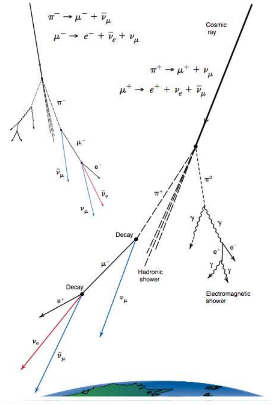
Figure 1.5 Cosmic rays produce extensive air showers upon collision with particles in the upper atmosphere, shown here. Muons and neutrinos are penetrating particles which can reach the IceCube detector through the overburden of ice or through the bulk of the Earth, respectively.
