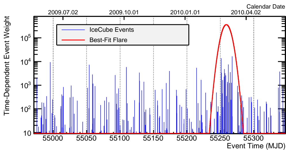
Figure 9.9 The event weights tested from the most significant flare location from the 59-string data at ( RA=21.35^\circ , \delta=-0.25^\circ ) and the best-fit spectral index of E^{-3.9} . The events are somewhat low-energy and roughly 1^\circ from the hottest location, only particularly standing out by virtue of their time structure. The best-fit Gaussian flare is shown in red.
