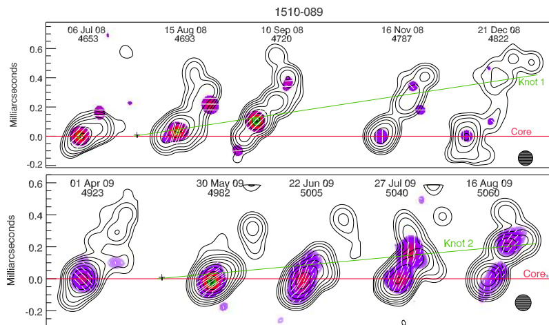
Figure 2.1 The motion of ejected blobs of material from the blazar PKS 1510-089 seen with 43 GHz radio images. The images are convolved with a circular Gaussian beam of the shaded circle at the lower right. Dates are given by calendar and with TJD (JD-2450000). The color shows the intensity of the polarization intensity. Figure from [38].
