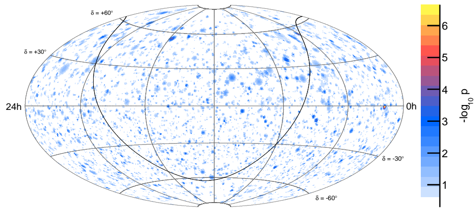
Figure 9.6 The map in equatorial coordinates of the pretrial p -value for the 59 string dataset all-sky flare search. The most significant flare can be seen in the center-right at 1h 25m, -0.25^\circ . The black curve is the Galactic plane.
