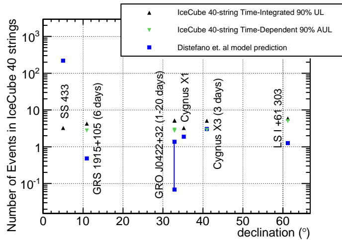
Figure 11.2 The time-integrated upper limit (UL) at 90% CL is compared to the expected number of events for model predictions according to [147] for specific sources for the 40 string configuration. The neutrino energy range used to calculate the total number of events is 10^8 - 5 \times 10^{14} eV, compatible to what assumed in the model. For non persistent but flaring sources, the parameters of the model were estimated for flares observed before IceCube construction. Hence the time-dependent upper limits are calculated averaging over a duration equal to the model flare during 40-string data taking (indicated as MUL in the legend). LS I +61° 303 is assumed to be a periodic flaring source in a high state during 26% of the orbit.
