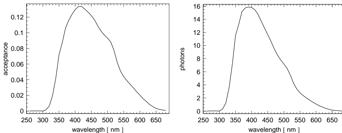
Figure 4.4 The plot on the left shows the acceptance of the DOM to photons traveling vertically upwards into the PMT versus wavelength. To the right shows the number of Čerenkov photons as a function of wavelength emitted per meter by a muon, convolved with the acceptance of the DOM. The integral of this curve is 2450 photons, the total number of photons emitted per meter.
