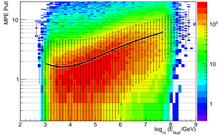
Figure 5.2 A plot of the uncorrected pull distribution of the MPE paraboloid reconstruction versus energy for the 40-string configuration. The pull is the reconstructed angular error divided by the true reconstruction error, so values larger than one indicate a reconstructed error which is too small. In practice, at higher energies stochastic energy losses along the track confuse the reconstruction, causing a narrower minimum than should be found. Finding a narrower minimum is much more detrimental to point-source analyses, as this will cause events which come from a common source to appear from separate sources, increasing the signal needed to make a discovery. Therefore we apply a correction, which is done as a fit to the median of the pull distribution shown here.
