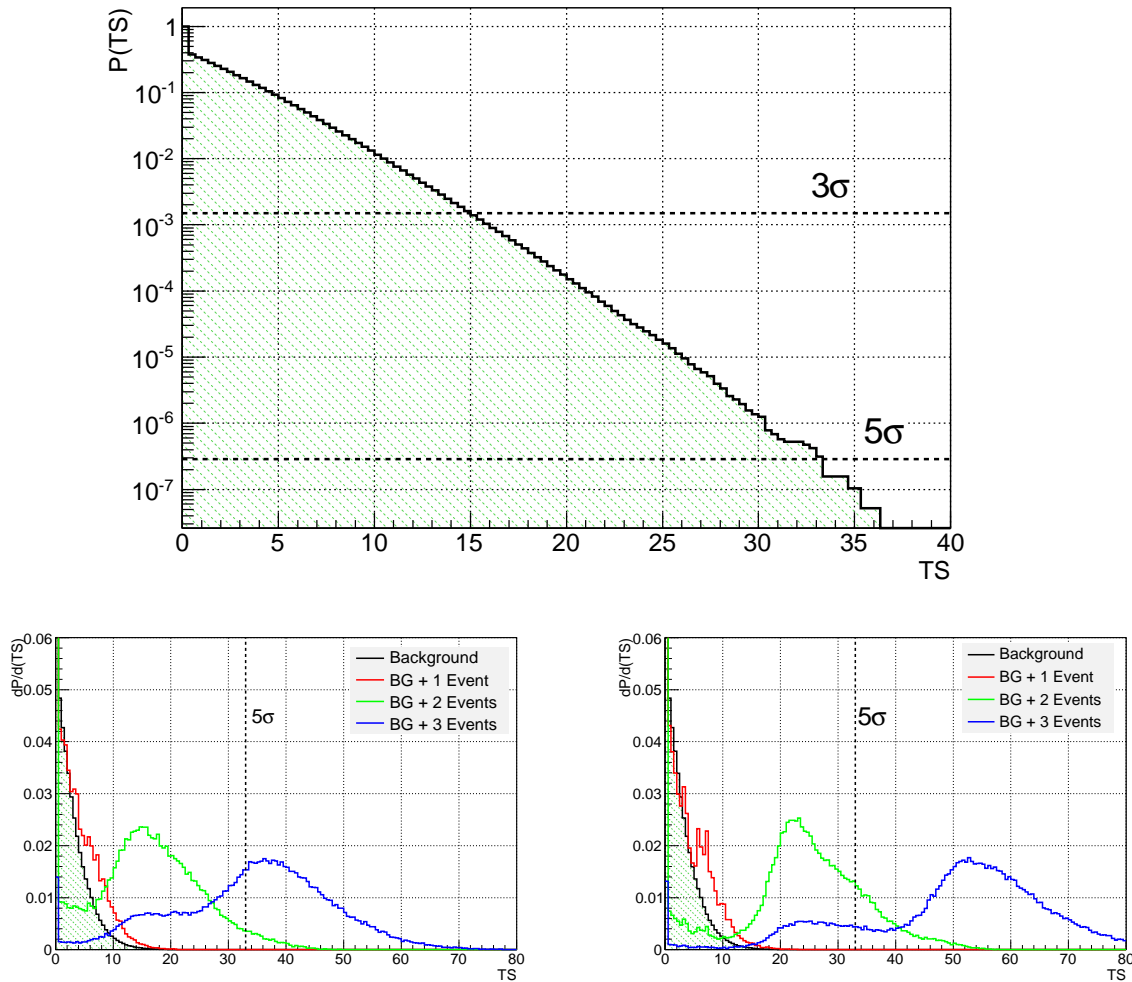
Figure 7.4 Integral distribution of the null test statistic distribution at \delta = +16.1^\circ with 3\sigma and 5\sigma thresholds indicated (top) following the untriggered search method described in Chapter 9. Below are the distributions of the test statistic for background and 1, 2 and 3 added signal events with a flare width of 15 minutes (bottom left) and 1, 2 and 3 added signal events with a flare width of 10 seconds (bottom right).
