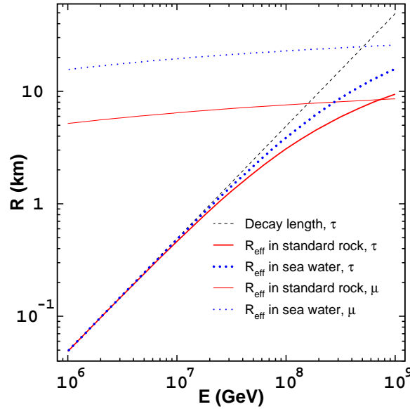
Figure 1.2 The mean range of high-energy muons and taus in rock and sea water. Figure from [5].
