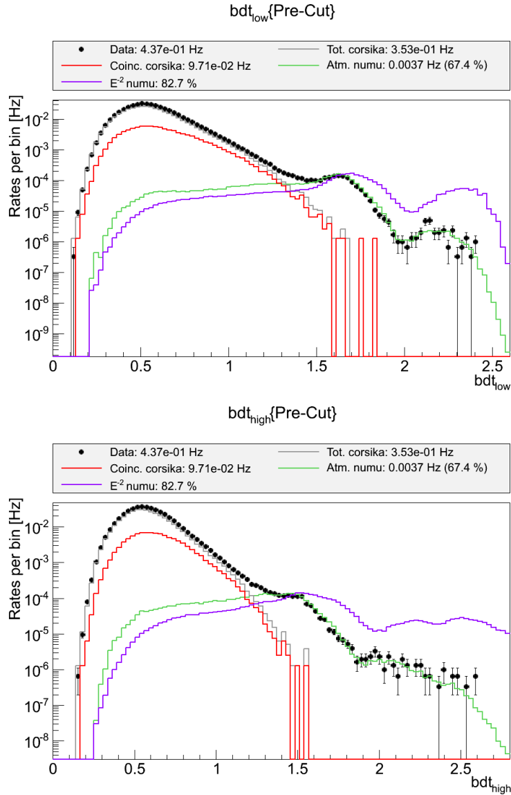
Figure 6.4 A graph of the BDT scores of events, where on the top is the score trained using an E^{-2.7} spectrum, and on the bottom is the score of the tree trained on an E^{-2} spectrum. Data is plotted as black dots, while signal and background simulations are drawn as lines for comparison.
