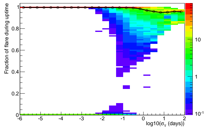
Figure 9.2 The fractional duration of randomly-simulated flares which occur during the uptime for the 40-string configuration for a range of different flare durations. The black line marks the median fraction of fluence occurring during the detector livetime for a given flare duration, which is used as a correction factor for the fluence of observed flares. For instance, for flares shorter than one minute, there is approximately an 8% chance of the flare occurring completely during detector downtime. Flares longer than one day will always have some emission during uptime; on average 92% of the total emission will coincide with usable run time.
