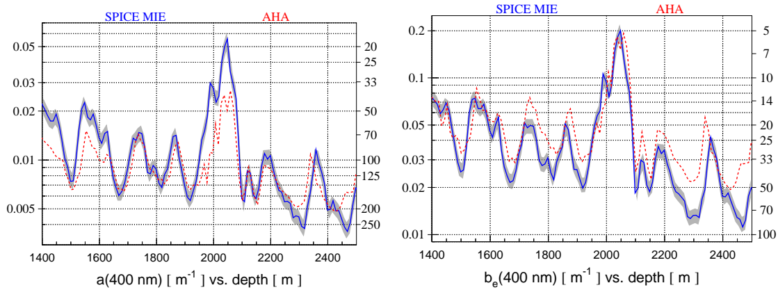
Figure 4.5 The fit parameters of the scattering length and absorption versus depth of the South Pole ice. Shown are two models of the ice properties: the AHA model which was first developed using flasher data from the AMANDA detector and extrapolated to the deep ice using dust logger data, and the SPICE MIE model which is more recent and uses an iterative fit with IceCube flasher data to model the dependence of the scattering and absorption versus depth.
