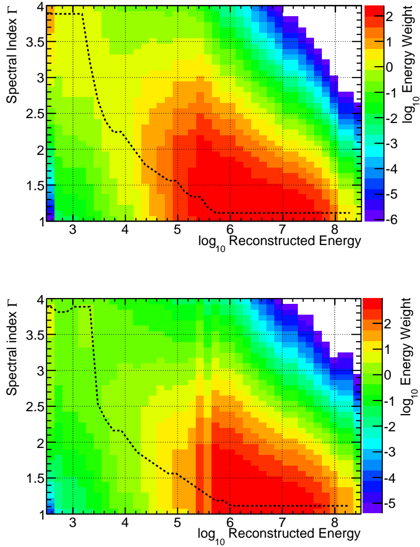
Figure 7.2 The energy weight S_i^{\text{energy}}(E_i, \theta_i, \gamma_s)/B_i^{\text{energy}}(E_i, \theta_i) for events near \theta_i = 106^\circ ( +16^\circ in declination), for the 40 and 59-string datasets (top and bottom, respectively). The dashed line indicates the spectral index which maximizes the ratio for a given reconstructed energy.
