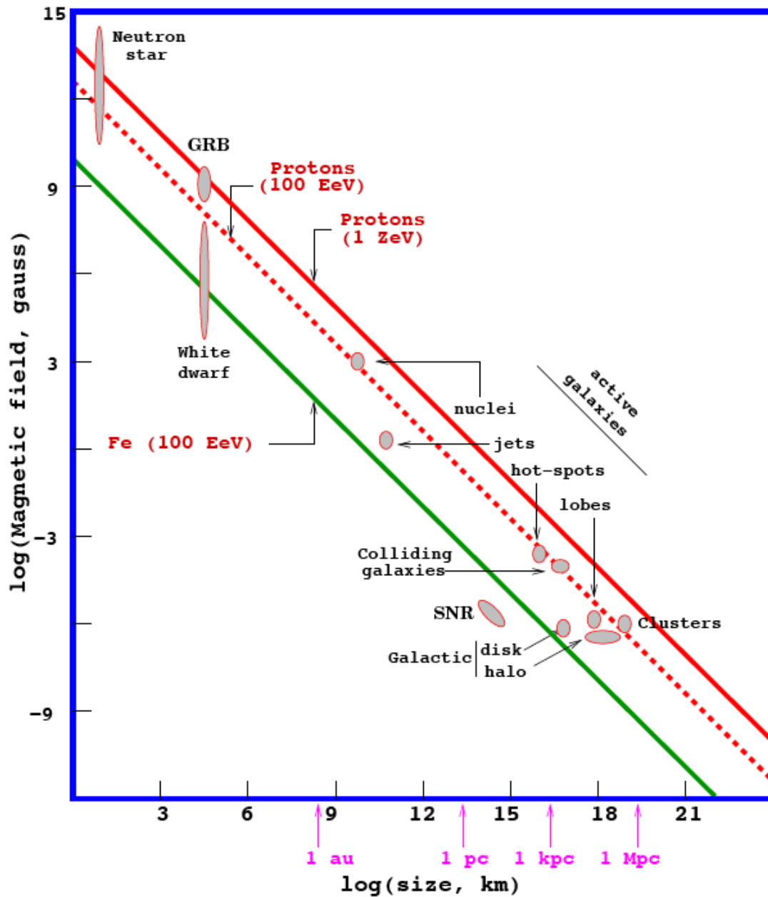
Figure 2.5 The Hillas plot of the distribution of source sizes and magnetic field strengths required to accelerate cosmic rays to specific energies for protons and iron, here marked off as the diagonal lines as the minimum size and magnetic field strength. Classes of astronomical objects which may be accelerators are marked. Plot from [91].
