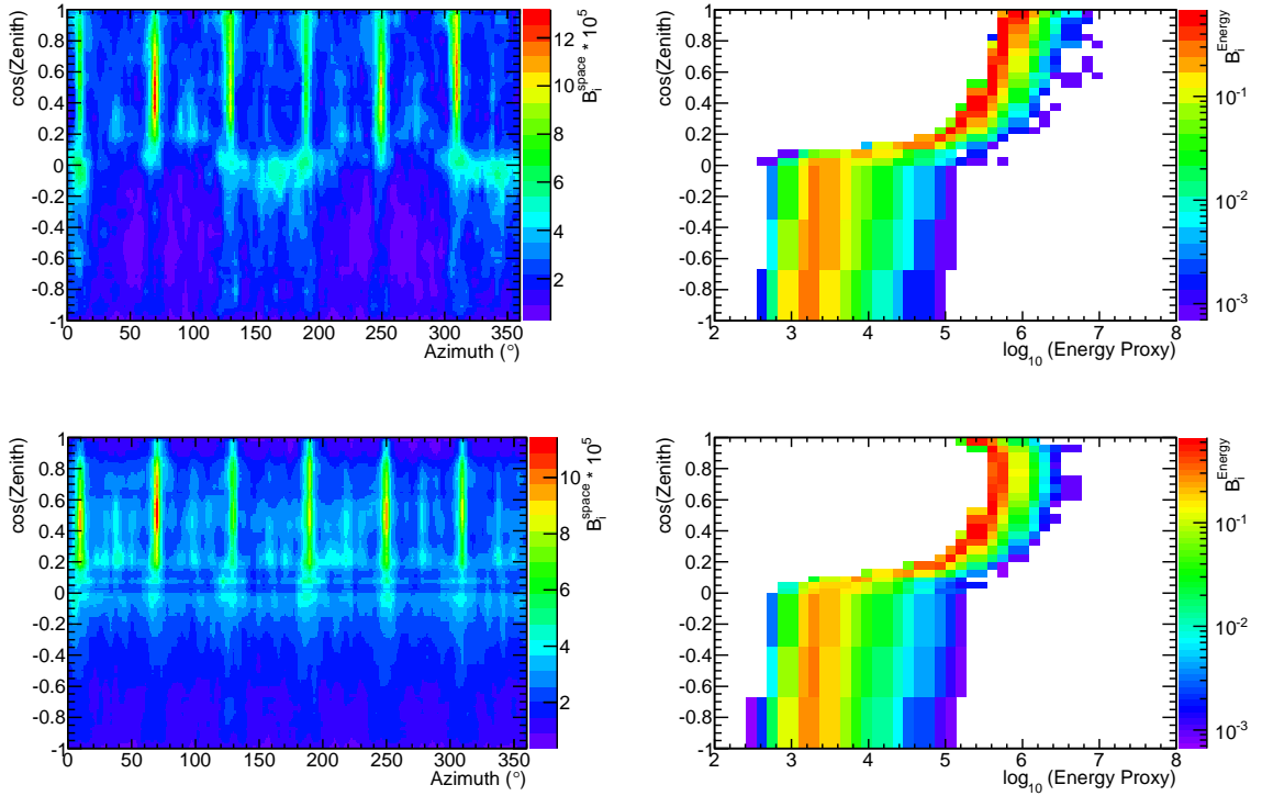
Figure 7.1 Above Left: The normalized event distribution of the 36,900 events in local coordinates for the 40 strings data (the space term in Equation 7.3). There are two predominant effects: for up-going events (northern sky, bottom half), events traveling down the longer end of the detector are more likely to trigger and pass cuts; for down-going events (southern sky, top half), there are six peaks in the event rate. This is due to the initial filter conditions at the South Pole that select tracks more efficiently when they pass close to aligned strings. Above Right: Normalized distribution of cosine of zenith as a function of the energy proxy E_{MuE} (the energy term in Equation 7.3). The lower row shows the same distribution for the 107,569 events selected for the 59 string sample. The two peaks for up-going events travelling down the long end of the 40-string detector is gone.
