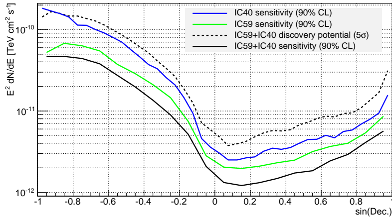
Figure 7.5 The time-integrated sensitivities to an E^{-2} spectrum muon neutrino signal plotted against declination for the 40- and 59-string configurations. The sensitivity and discovery potential are also plotted for the combined dataset.
