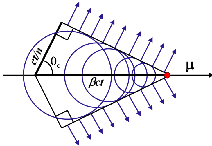
Figure 1.3 Illustration of Čerenkov emission. While a particle travels \beta ct in a time t , its emitted light only travels ct/n , forming a coherent front in a cone around the direction of motion. Use of this directionality is used in the reconstruction of the particle's properties.
