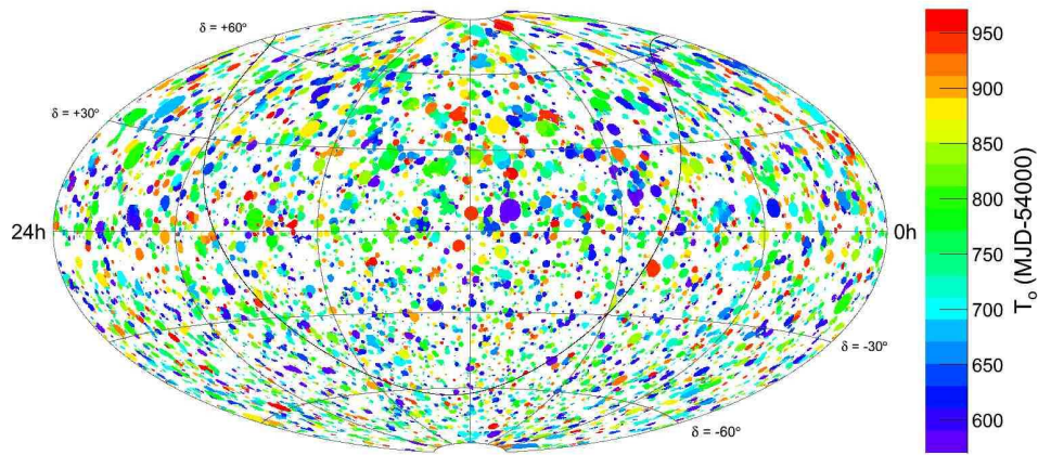
Figure 9.4 The equatorial coordinate map shows the best fit of the mean time of the flare \hat{T}_o (MJD-54,000) for the most significant flare during the 40-string data taking period found at each location of the grid where the likelihood is calculated. The black curve is the Galactic plane.
