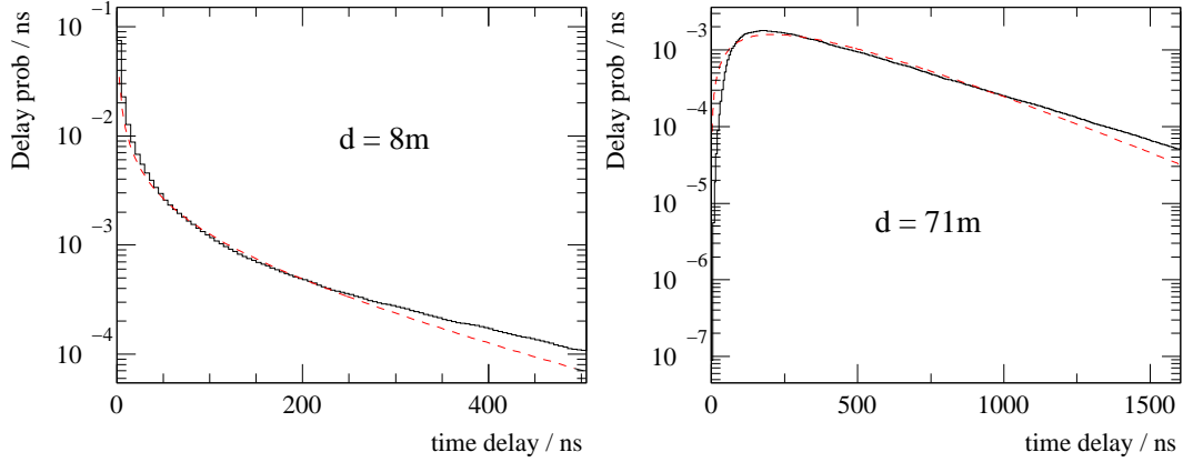
Figure 5.1 Diagrams of the time residual distribution using the Pandel function (dashed curves) to the detailed simulation (in black) at two distances from the simulated muon track.
