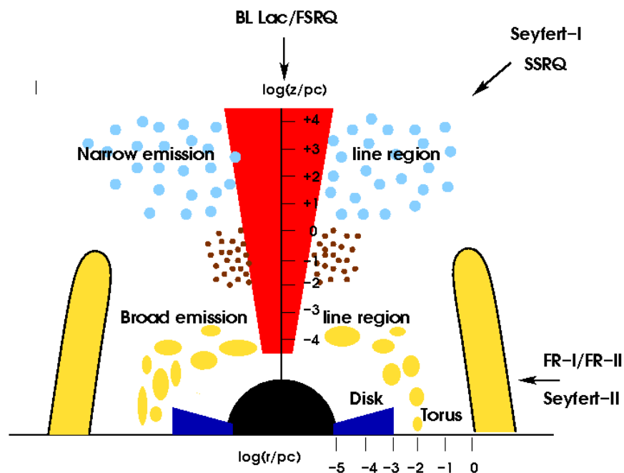
Figure 2.2 Schematic of a cylindrically-symmetrical center of an AGN. Axes are logarithmic in units of parsec. Regions of the AGN are marked. The classification of an AGN are marked off by arrows approximating the viewing angle of the observer. Figure from [7].
