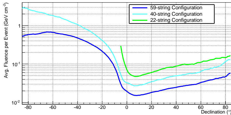
Figure 7.6 The normalization per event on the fluence from an E^{-2} spectrum muon neutrino signal in a declination band divided by the number of events in the band in the 22, 40 and 59-string configurations, plotted against declination.
